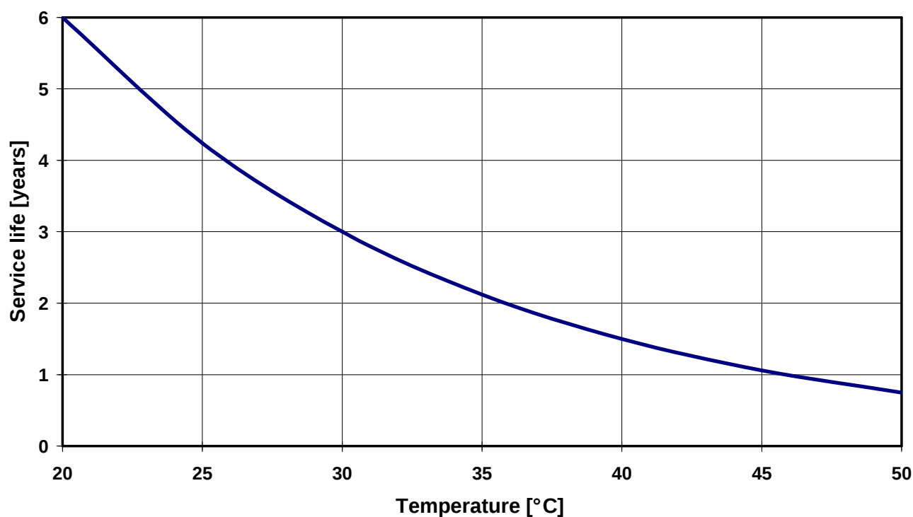
Fig. 30: A500 - Service Life vs. Temperature (following law of “Arrhenius”).
