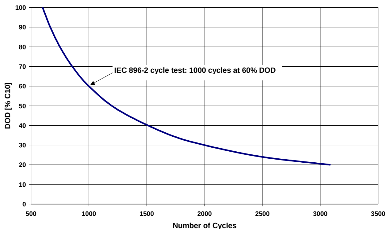
Fig. 21: A600 block - Number of Cycles vs. Depth of Discharge (DOD)
