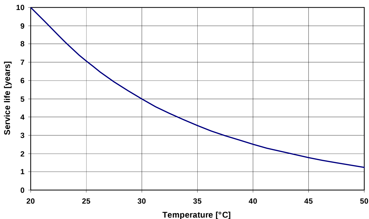
Fig. 31: A400 - Service Life vs. Temperature (following law of “Arrhenius”)
