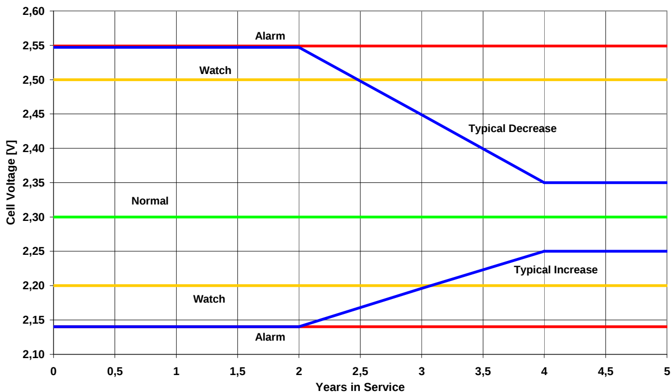
Fig. 8: A500 (2 V) – Float Voltage Deviation vs. Years
