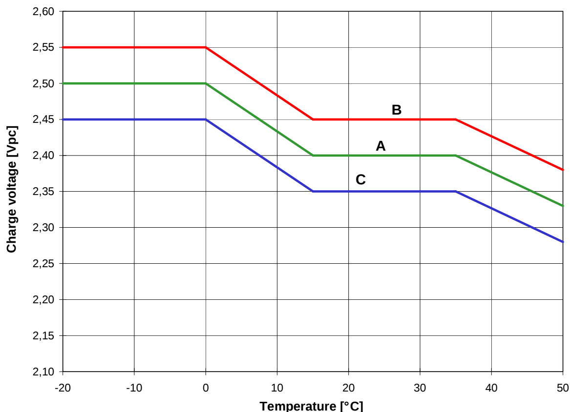
Fig. 26: Charging of Gel-Solar-batteries depending on Charge Mode and Temperature:
